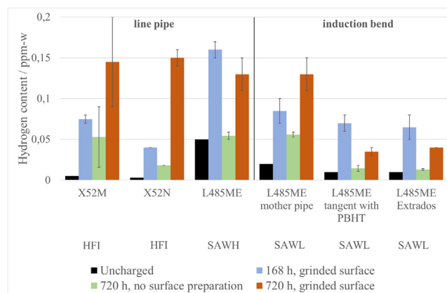
Fig. 2. Results of immersion tests for different steel grades/products.
